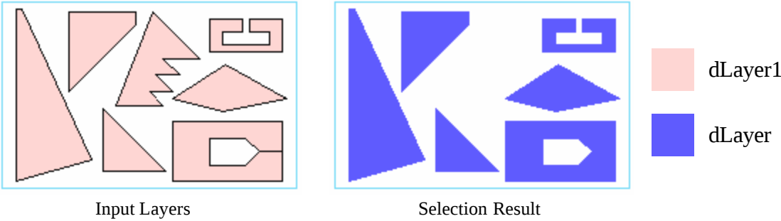
例2 : Non Obvious
