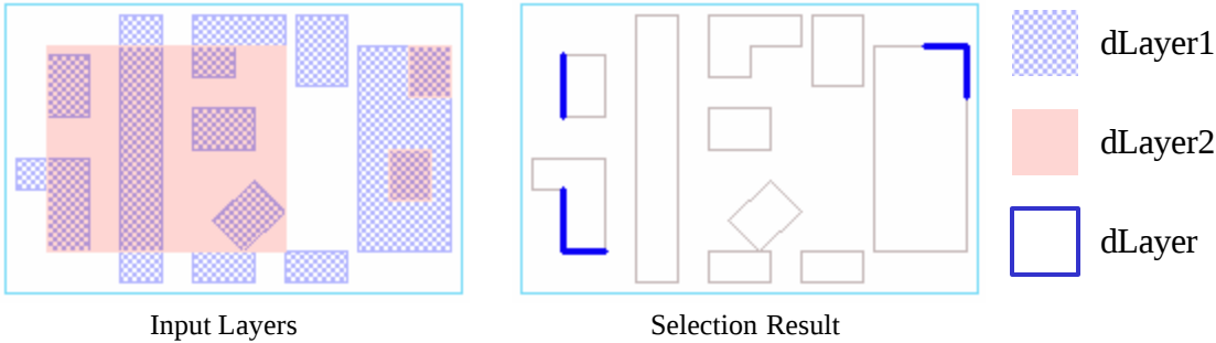
例1 : Obvious
