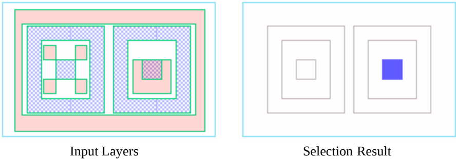
例2 : Non Obvious
